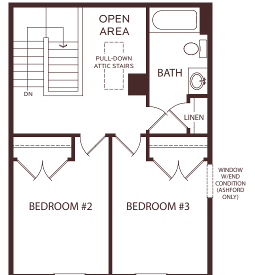
3 RD LEVEL WITH TWO BEDROOMS, OPEN AREA
