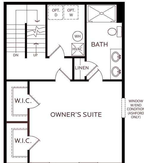
2 ND LEVEL WITH STANDARD BATH, TWO WALK-IN CLOSETS (SK-4)
